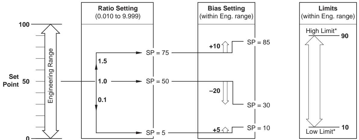
Fig. 4.2 Set Point Types
